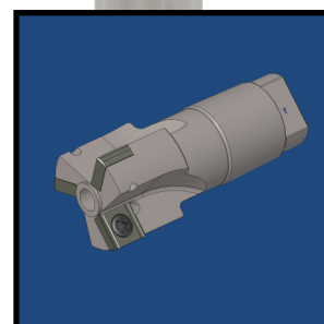
MODULAR FRONT COUNTERBORING
