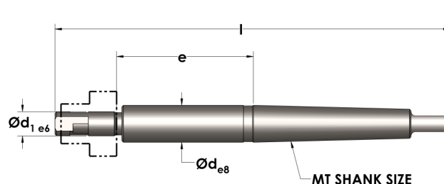
TUH Holder Morse Taper Shank
