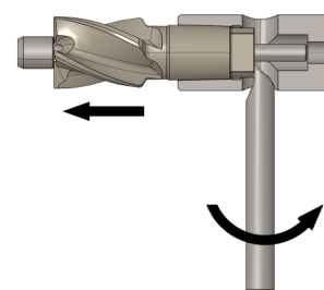
EJECTOR H FOR COUNTERBORE WITH PILOT
