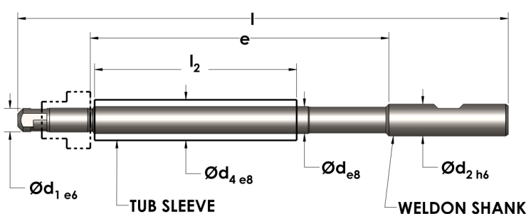
TUHW Holder Weldon Shank With TUB Bushing
