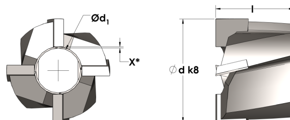
TU Cutter Head Carbide
