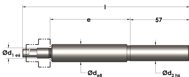
TUH Holder Cylindrical Shank
